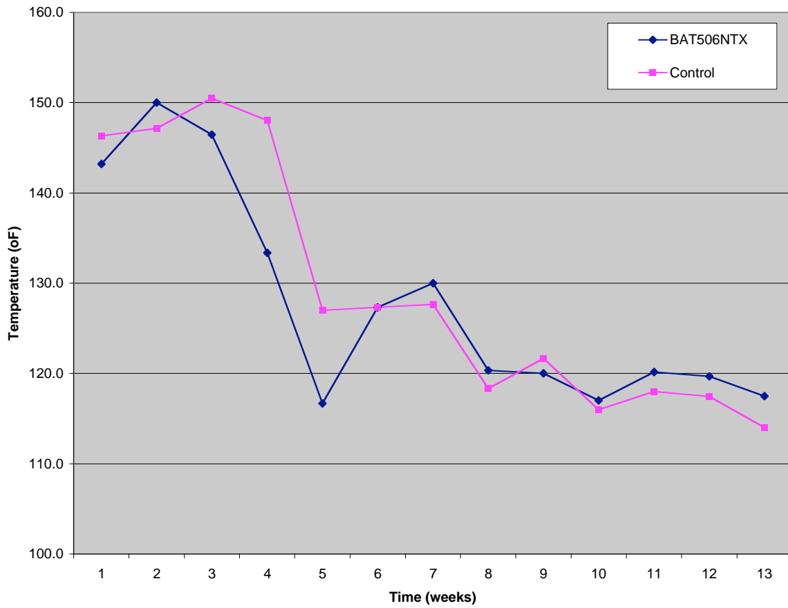
Figure 5. Temperatures Readings Pilot Project BAT506NTX R&D Soil Builders
